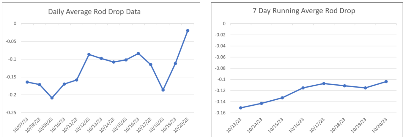
Figure 5 – Trend Plots Showing a Daily Average and a 7-Day Running Average of Rod Drop Values
